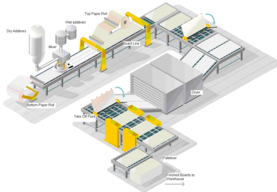
Manufacturing process flow diagram
